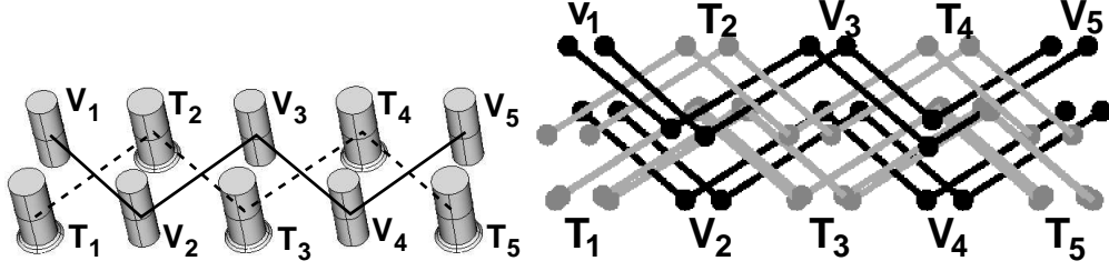
Figure 11: \mathbf{Z} regularity and location cycles for \{(V_1, V_2, \dots, V_5), (T_1, T_2, \dots, T_5)\} detected in the Angle Bracket after RFT construction
