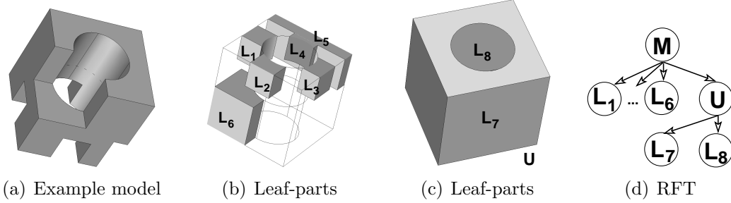
Figure 18: A four-fold rotational symmetric arrangements was not detected due to the interpretation of RFT construction
