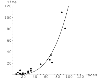
Figure 7. Algorithm performance
