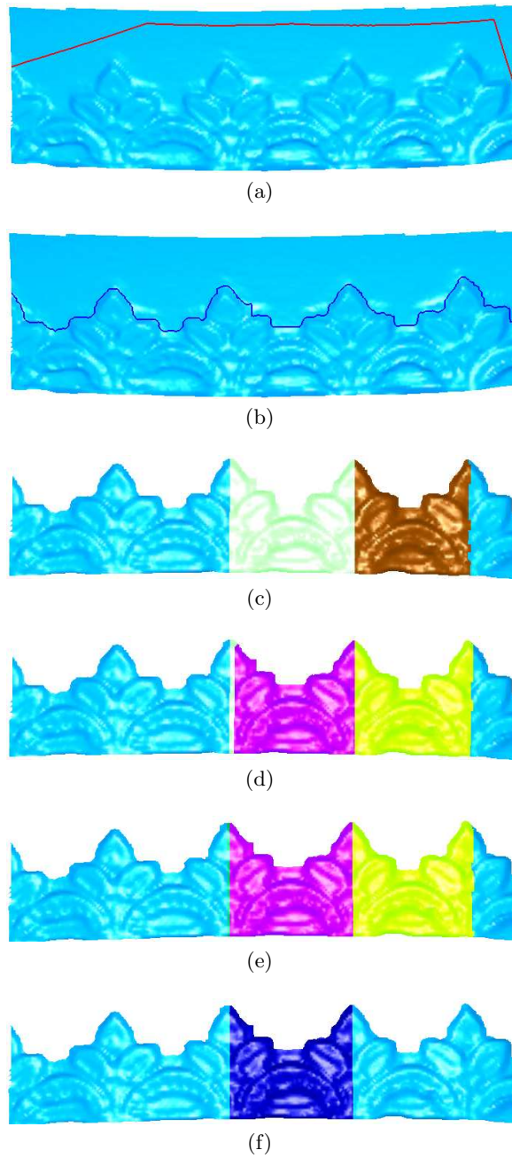
Fig. 5. Periodic relief segmentation for an example with leaves: (a) mesh model and the initial contour, (b) extracted relief boundaries by snake evolution, (c) units separated from coarse extraction phase, (d) results from refinement phase, (e) results from localization phase, (f) final extracted unit
