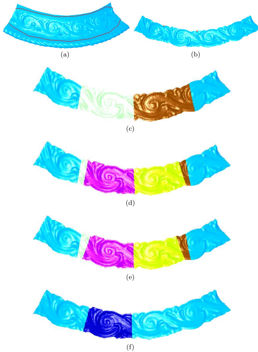
Fig. 6. Periodic relief segmentation without using boundary repetitive extraction: (a) mesh model and the initial contour, (b) user-specified corresponding points, (c) units separated from coarse extraction phase, (d) results from refinement phase, (e) results from localization phase, (f) final extracted unit
